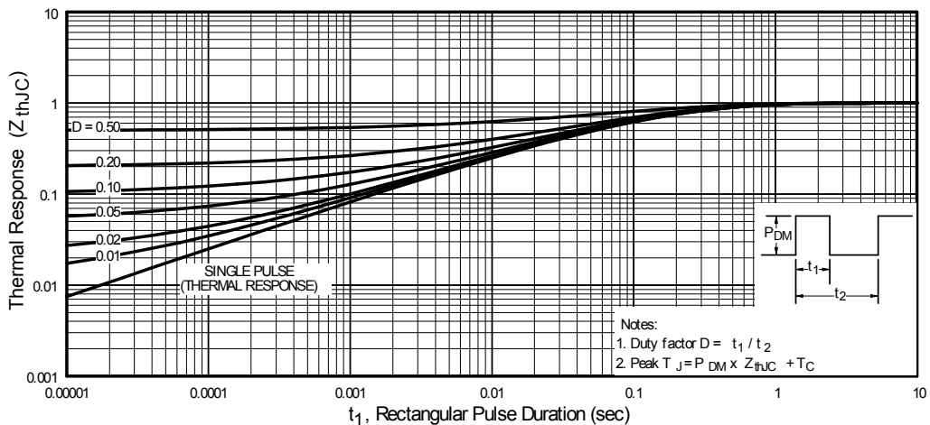
Fig. 4 Max. Thermal Impedance Z_{thJC} Characteristics
