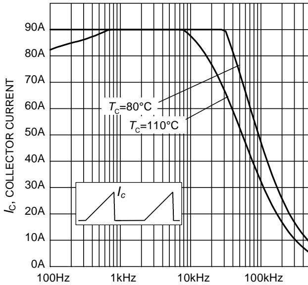
Figure 1. Collector current as a function of switching frequency for triangular current ( E_{on} = 0 , hard turn-off) ( T_j \leq 175^\circ\text{C} , D = 0.5 , V_{CE} = 400\text{V} , V_{GE} = 0/15\text{V} , r_G = 10\Omega )
