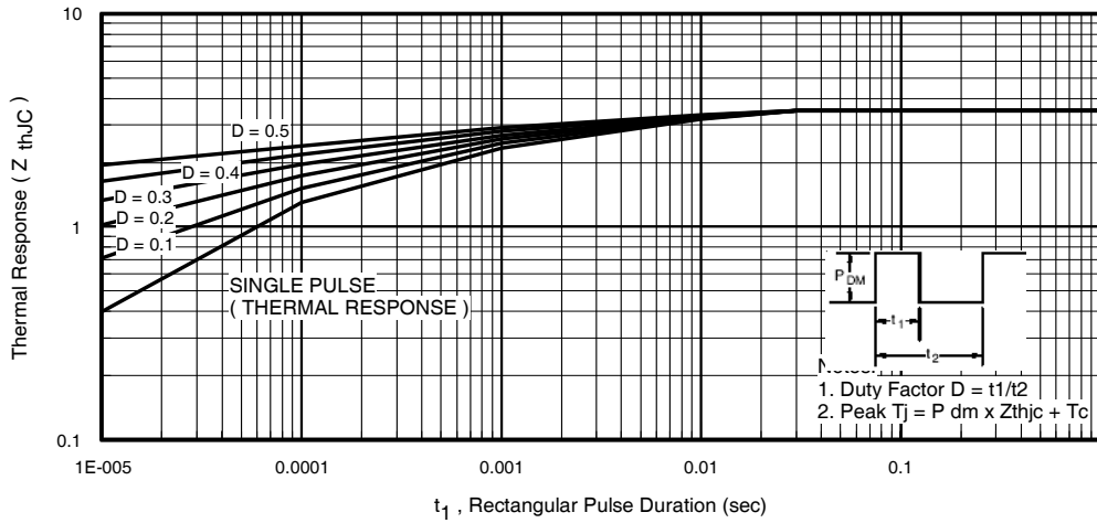
Fig. 4 - Max. Thermal Impedance Z_{thJC} Characteristics (Per Leg)
