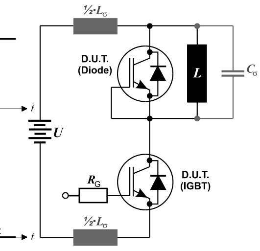
Figure E. Dynamic test circuit
