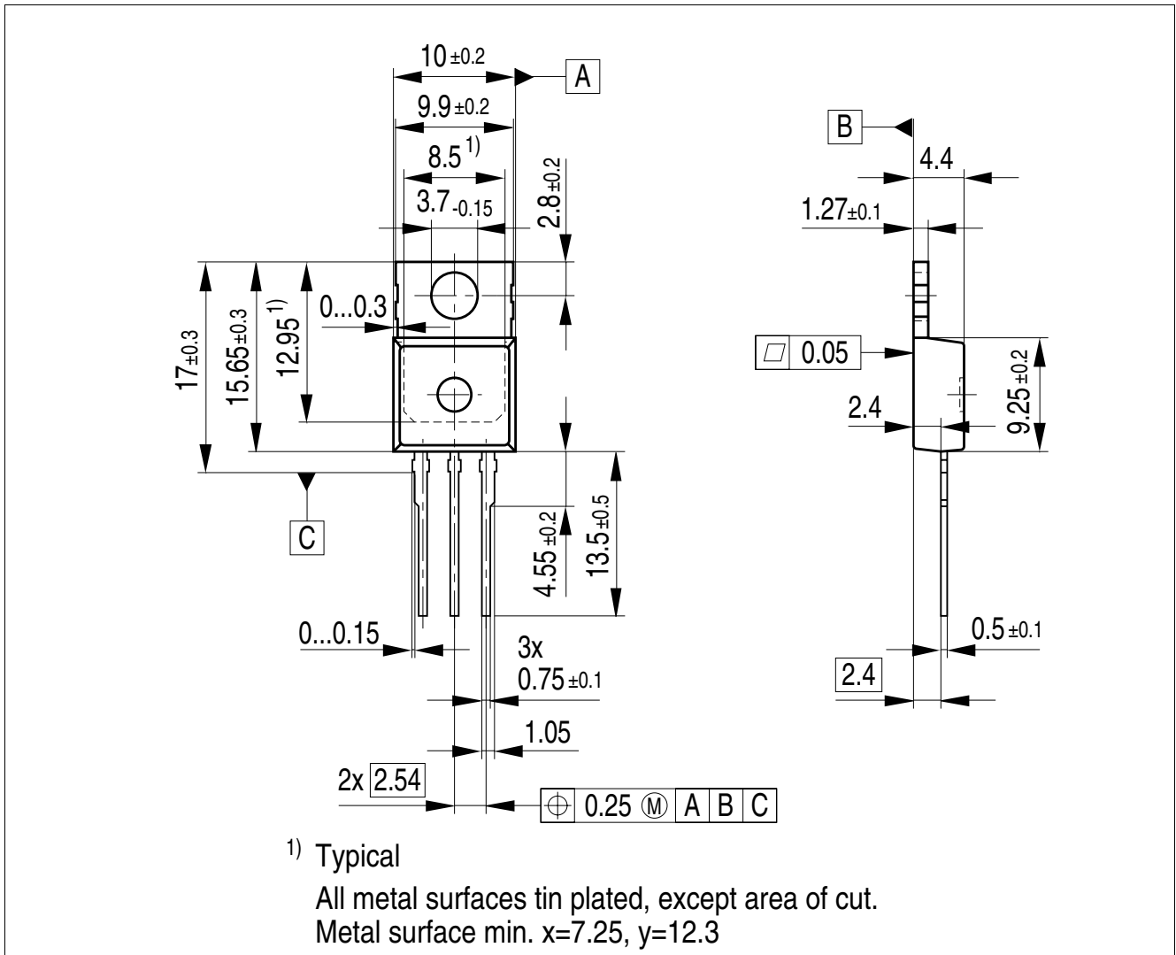
Figure 5 PG-T0220-3
