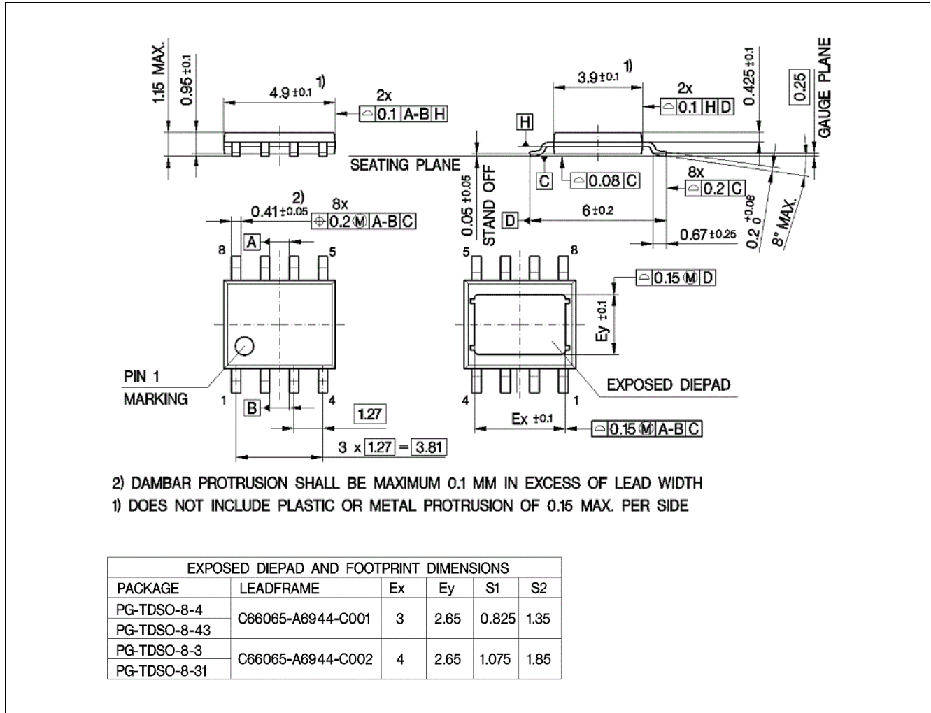
Figure 47 PG-TDSO8-31
