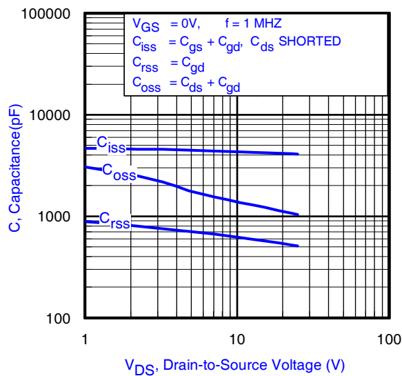
Fig 8. Typical Capacitances vs. Drain-to-Source Voltage
