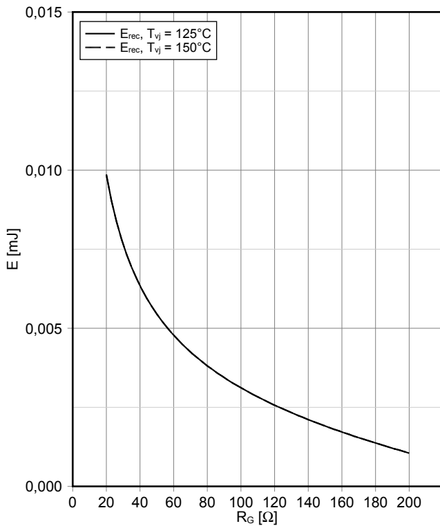
Schaltverluste Diode, 3-Level (typisch) switching losses Diode, 3-Level (typical) E_{rec} = f(R_G) I_F = 10 \text{ A}, V_{CE} = 300 \text{ V}
