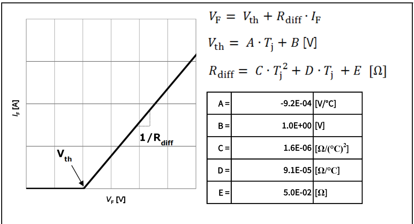
Figure 6 Simplified forward characteristics model V_F = f(I_F) ; -40°C < T_j < 175°C; I_F < 16 A
