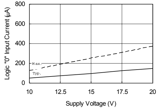
Figure 31B. Logic "0" Input Bias Current vs. Supply Voltage
