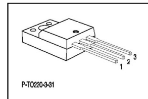
PG-TO220-3-31
