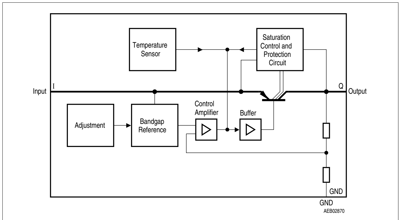
Figure 1 Block diagram
