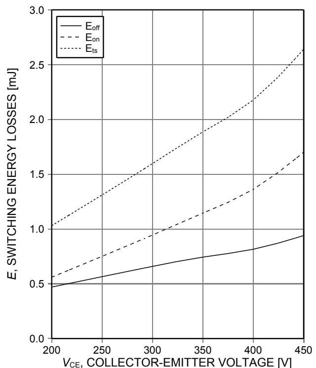
Figure 16. Typical switching energy losses as a function of collector emitter voltage (ind. load, T_J=175^{\circ}\text{C} , V_{GE}=15/0\text{V} , I_c=40\text{A} , r_G=7,9\Omega , test circuit in Fig. E)
