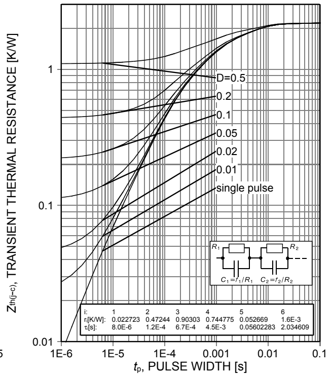
Figure 2. Diode transient thermal impedance per diode as a function of pulse width ( D = t_p/T )
