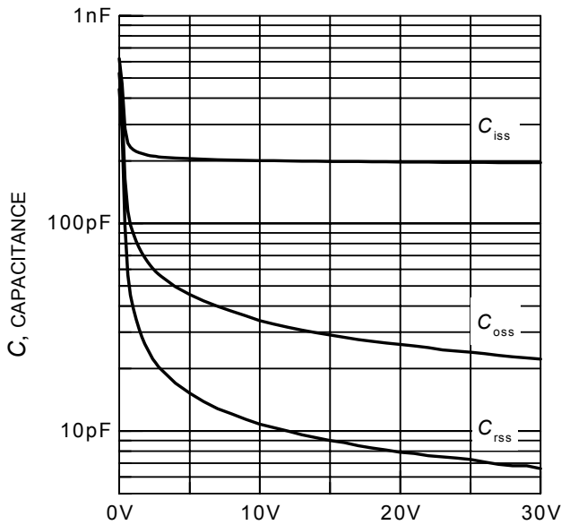
Figure 19. Typical capacitance as a function of collector-emitter voltage ( V_{GE} = 0V, f = 1MHz )
