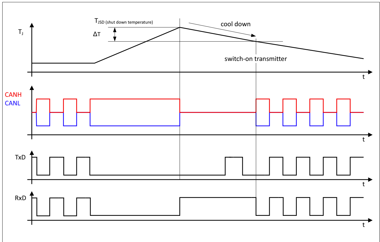
Figure 8 Overtemperature protection
