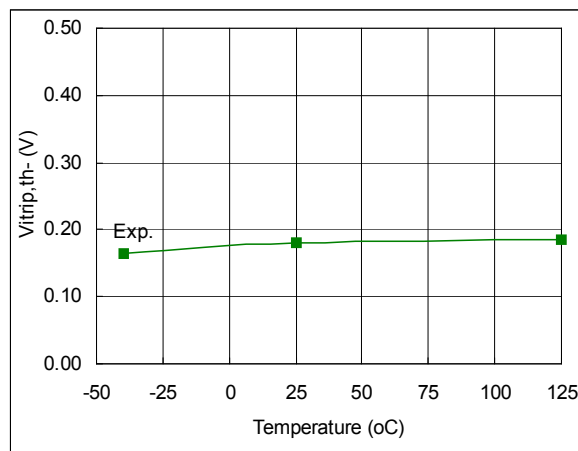
Fig. 99. Input Negative Going Threshold vs. Temperature
