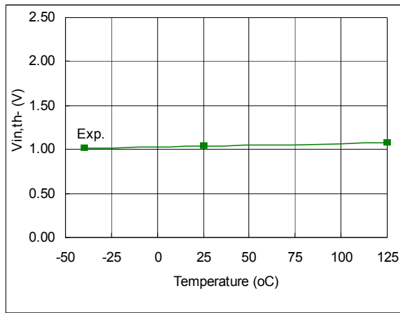
Fig. 97. Input Negative Going Threshold vs. Temperature
