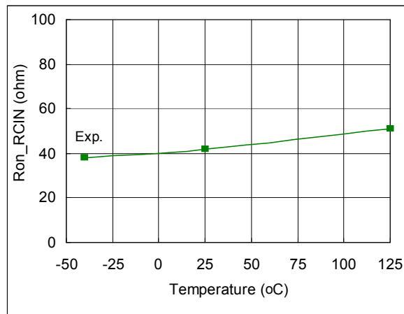
Fig. 95. RCIN Low On Resistance vs. Temperature
