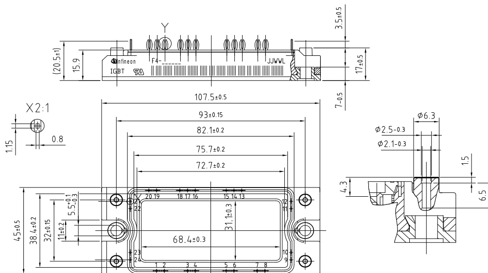
PCB hole pattern
