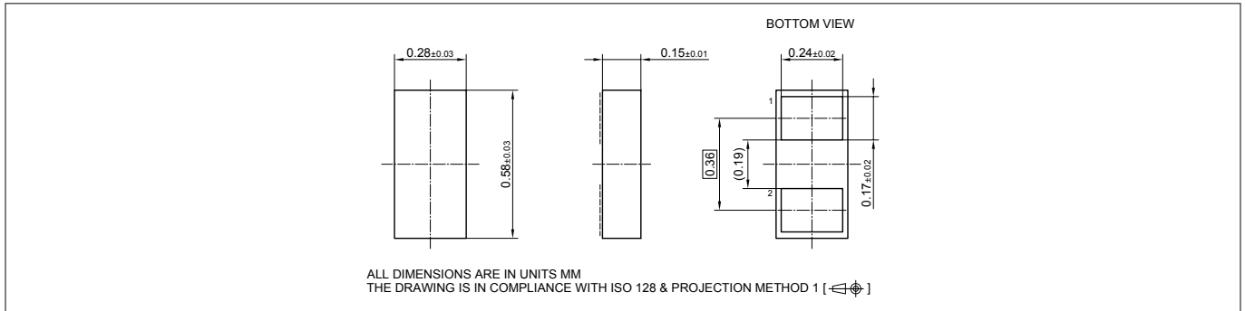
Figure 12 WLL-2-3 package outline
