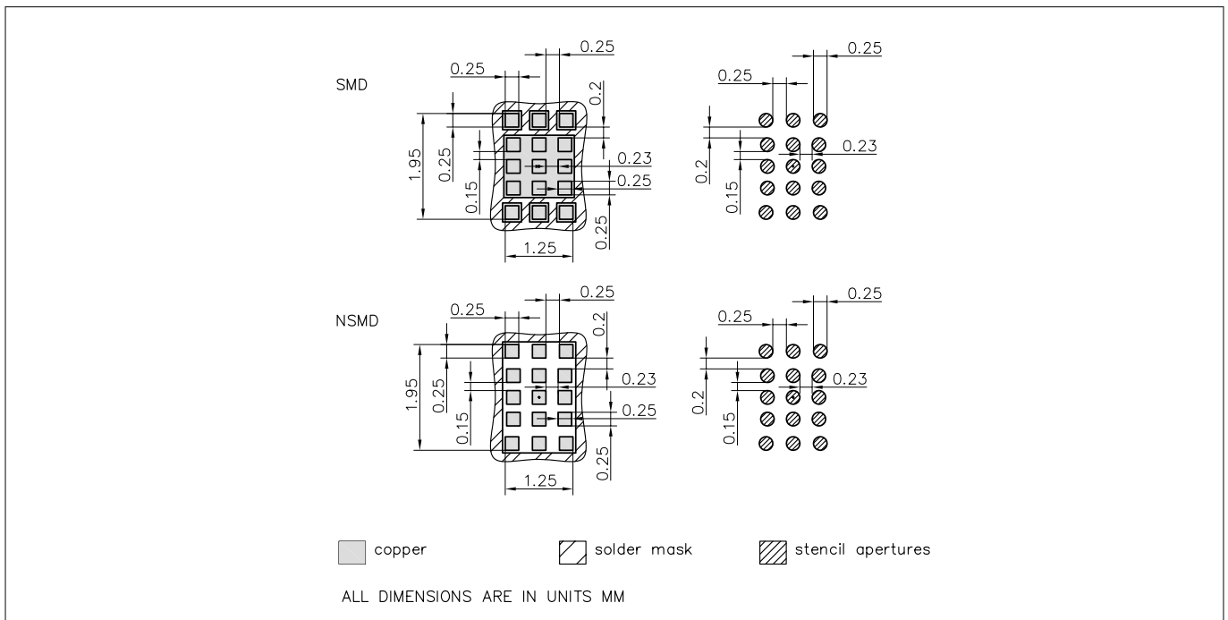
Figure 17 Foot print
