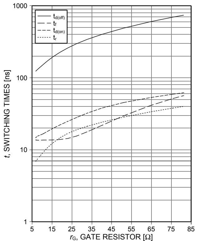
Figure 8. Typical switching times as a function of gate resistor (inductive load, T_{vj}=150^\circ\text{C} , V_{CE}=400\text{V} , V_{GE}=15/0\text{V} , I_c=20\text{A} , Dynamic test circuit in Figure E)
