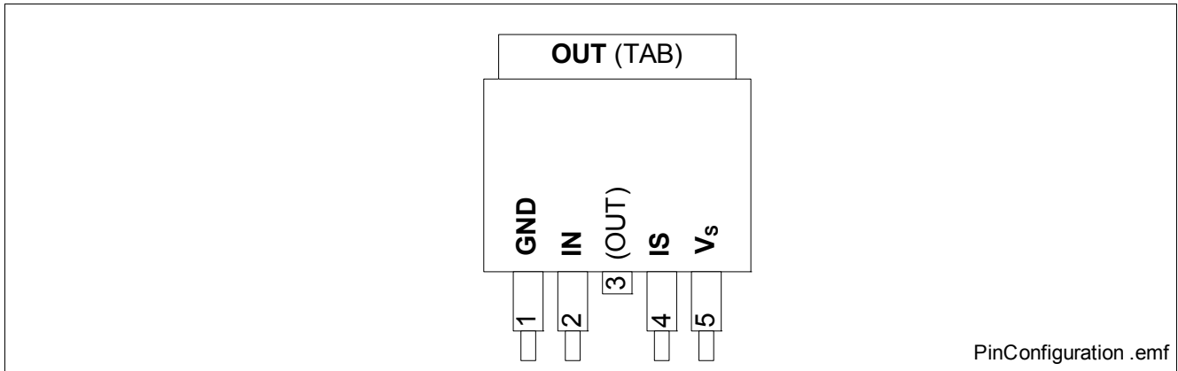
Figure 2 Pin Configuration
