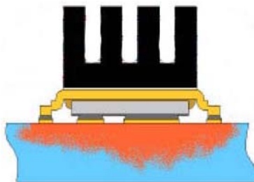
⑧ Mounted on minimum footprint full size board with metalized back and with small clip heatsink. (still air)
