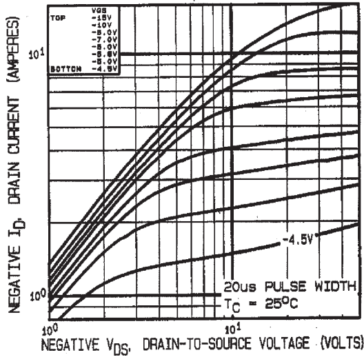
Fig 14. Typical Output Characteristics
