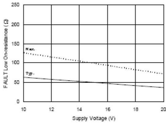
Figure 39B. FAULT Low On-resistance vs. Supply Voltage
