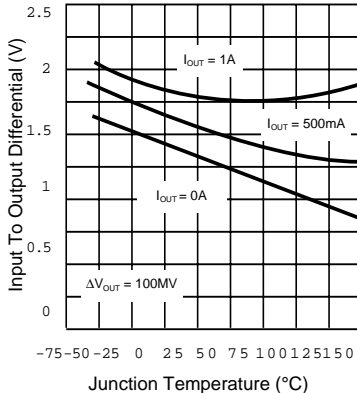
DROPOUT VOLTAGE
