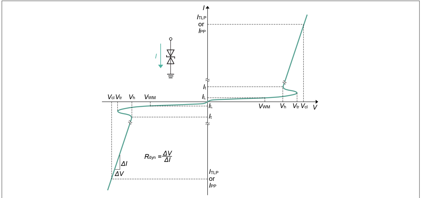
Figure 2 Definitions of electrical characteristics
