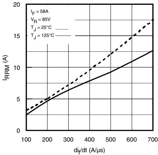
Fig. 18 - Typical Recovery Current vs. di/dt
