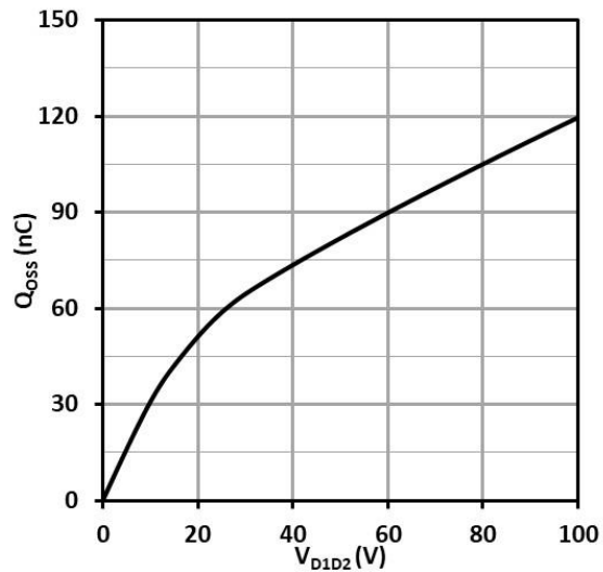
Fig. 14 Output Charge
