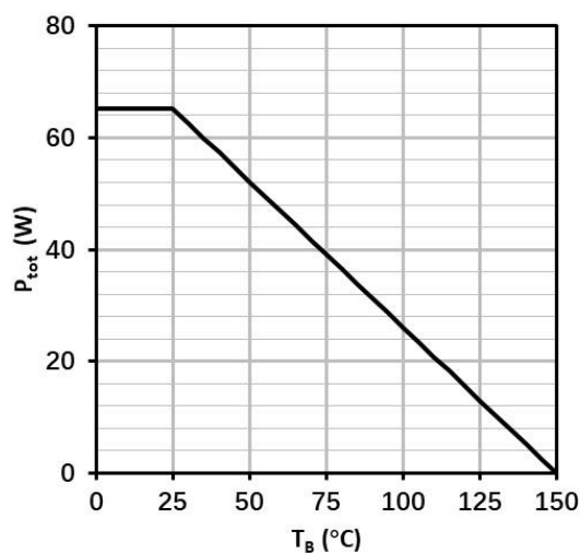
Fig. 16 Power Dissipation
