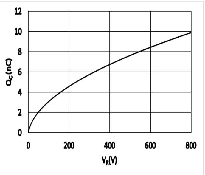
Figure 4. Recovery Charge vs. Reverse Voltage
