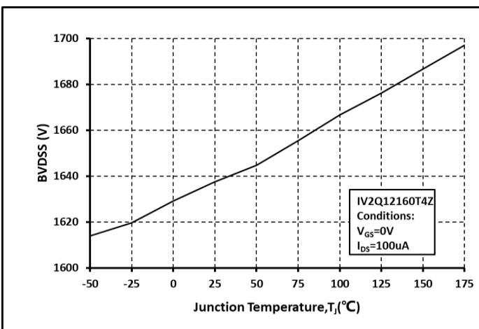
Fig. 27 BVdss vs. Temperature
