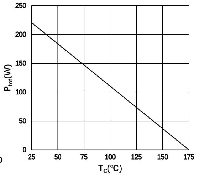
Figure 6. Power Derating
