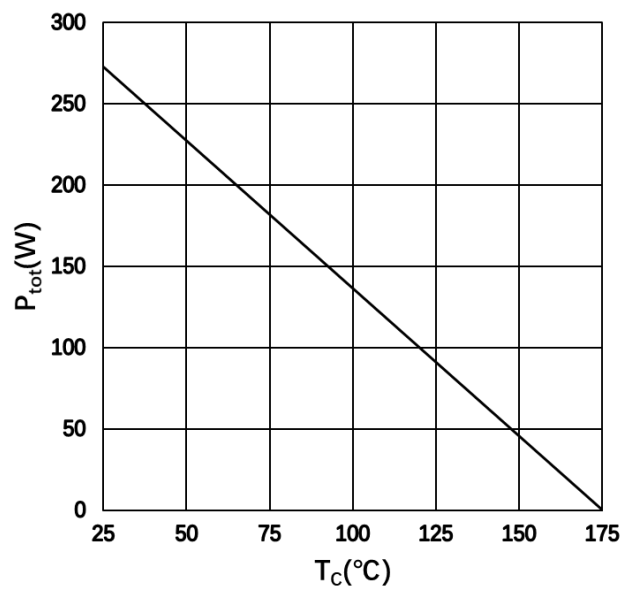
Figure 6. Power Derating
