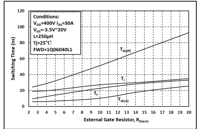
Fig. 20 Switching Times vs. R_{G(ext)}
