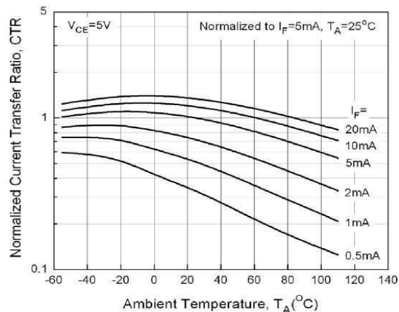
Fig 8 Normalized CTR vs Ambient Temperature
