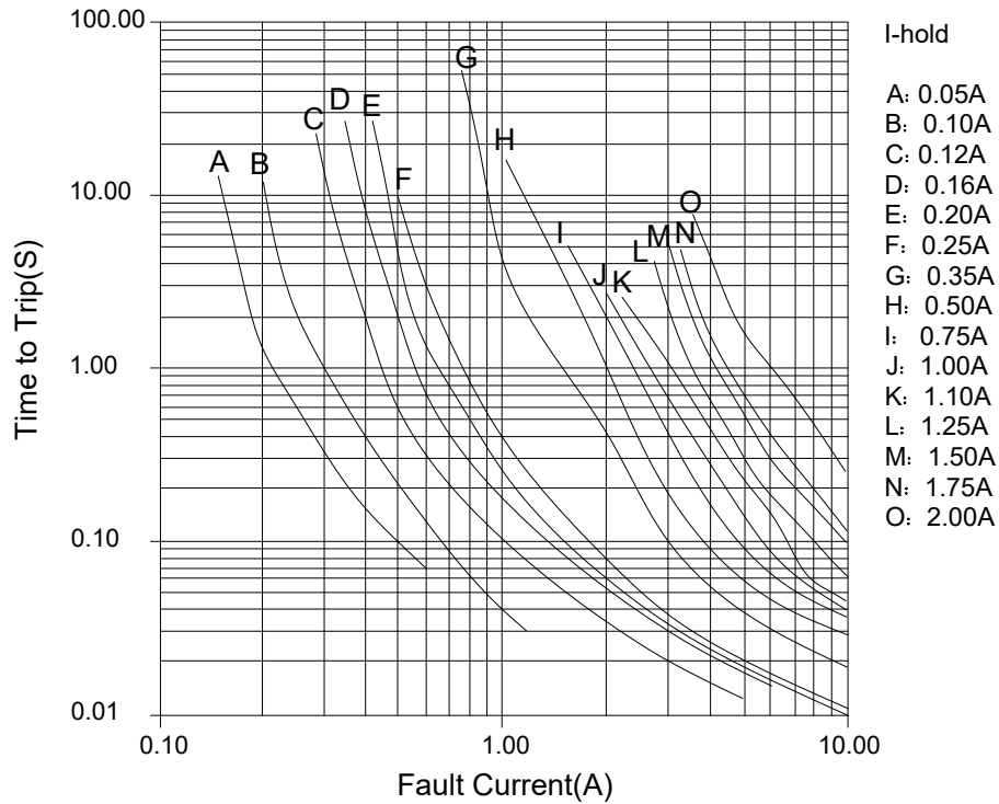
1206 Series TTT Vs Fault current chart
