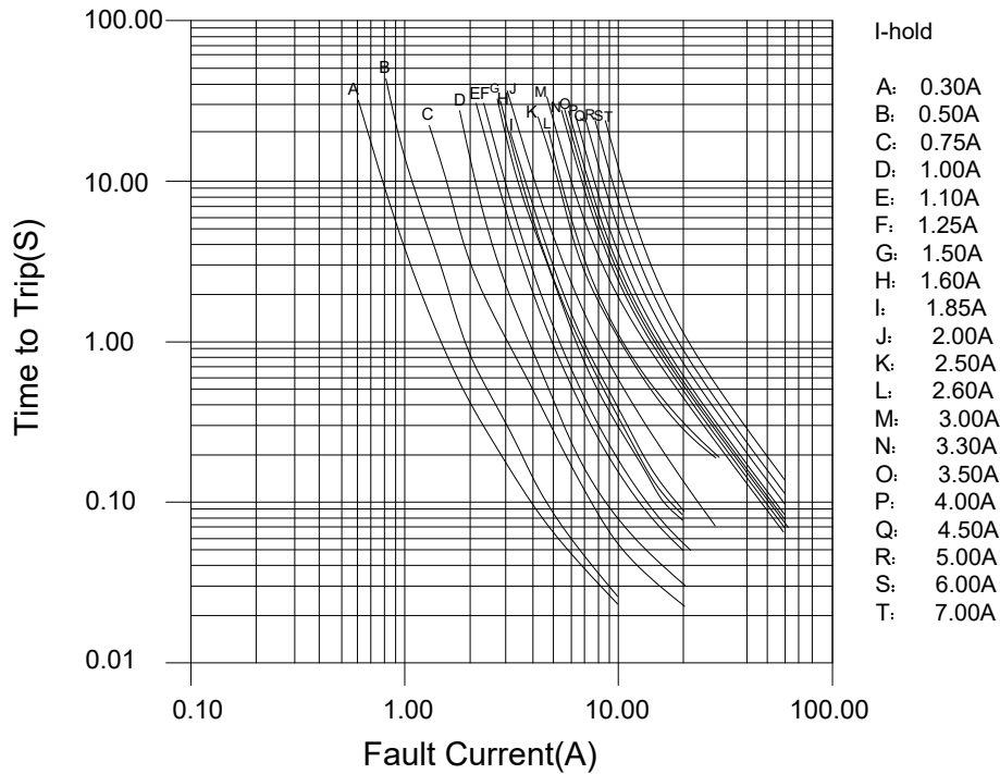
2920 Series TTT Vs Fault current chart
