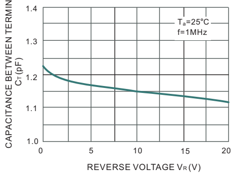
Fig.4 Capacitance Characteristics
