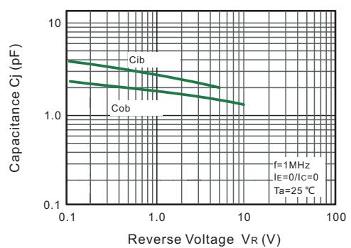
Fig.8 Cob/Cib-VCE/VBE
