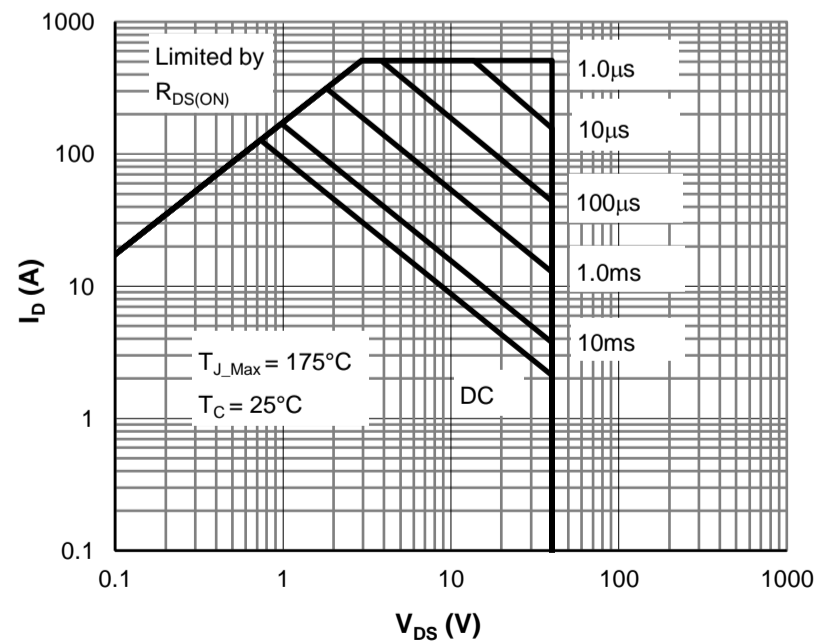
Figure 12: Maximum Safe Operating Area
