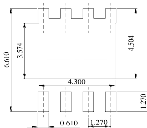
DIMENSIONS: MILLIMETERS
