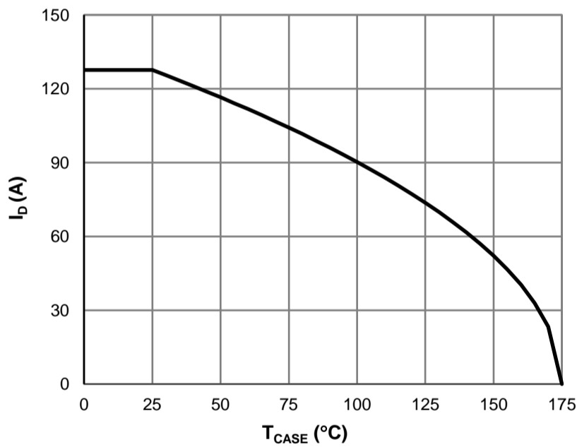
Figure 9: Current De-rating
