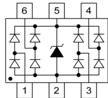
PIN Configuration
