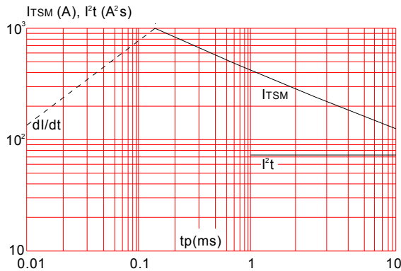
FIG.5: Non-repetitive surge peak on-state current for a sinusoidal pulse with width tp<10ms, and corresponding value of I²t (di/dt < 50A/μs)
