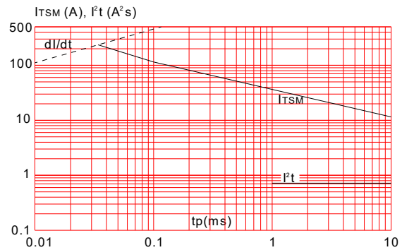
FIG.6: Non-repetitive surge peak on-state current for a sinusoidal pulse with width t_p < 10\text{ms} , and corresponding value of I^2t ( dI/dt < 50\text{A}/\mu\text{s} )
