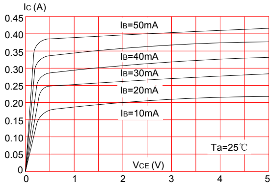
FIG.3: Base current vs. collector emitter saturation voltage
