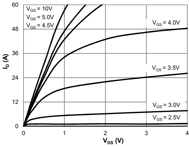
Figure 1: Saturation Characteristics
