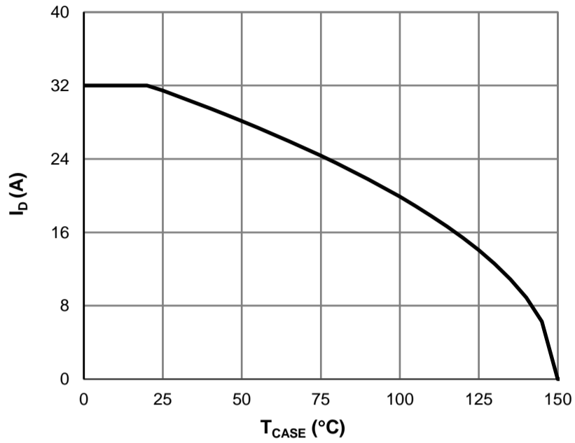
Figure 7: Current De-rating
