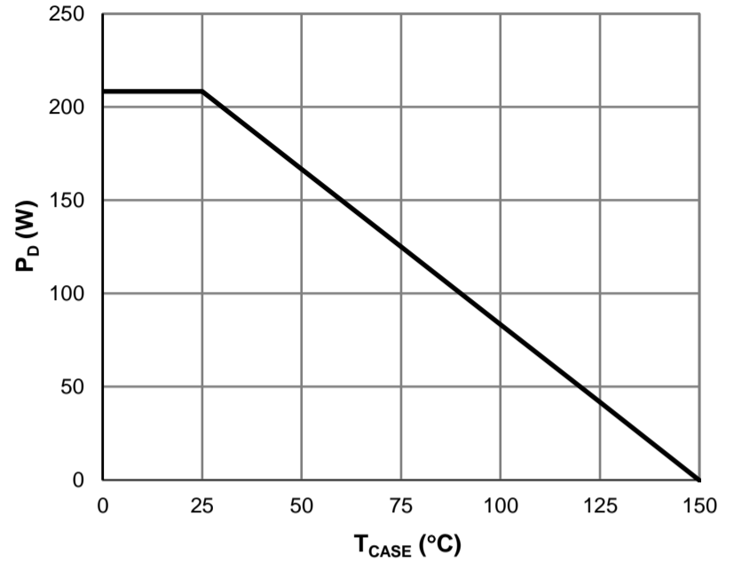
Figure 8: Power De-rating
