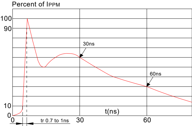
FIG.4: ESD clamping (15kV contact)
