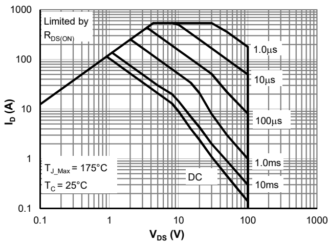
Figure 9: Maximum Safe Operating
