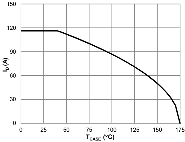
Figure 7: Current De-rating
