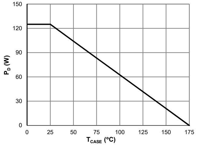
Figure 8: Power De-rating
