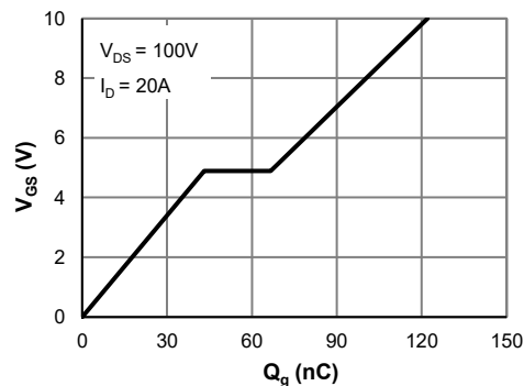
Gate Charge
