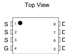
Pin Configuration
